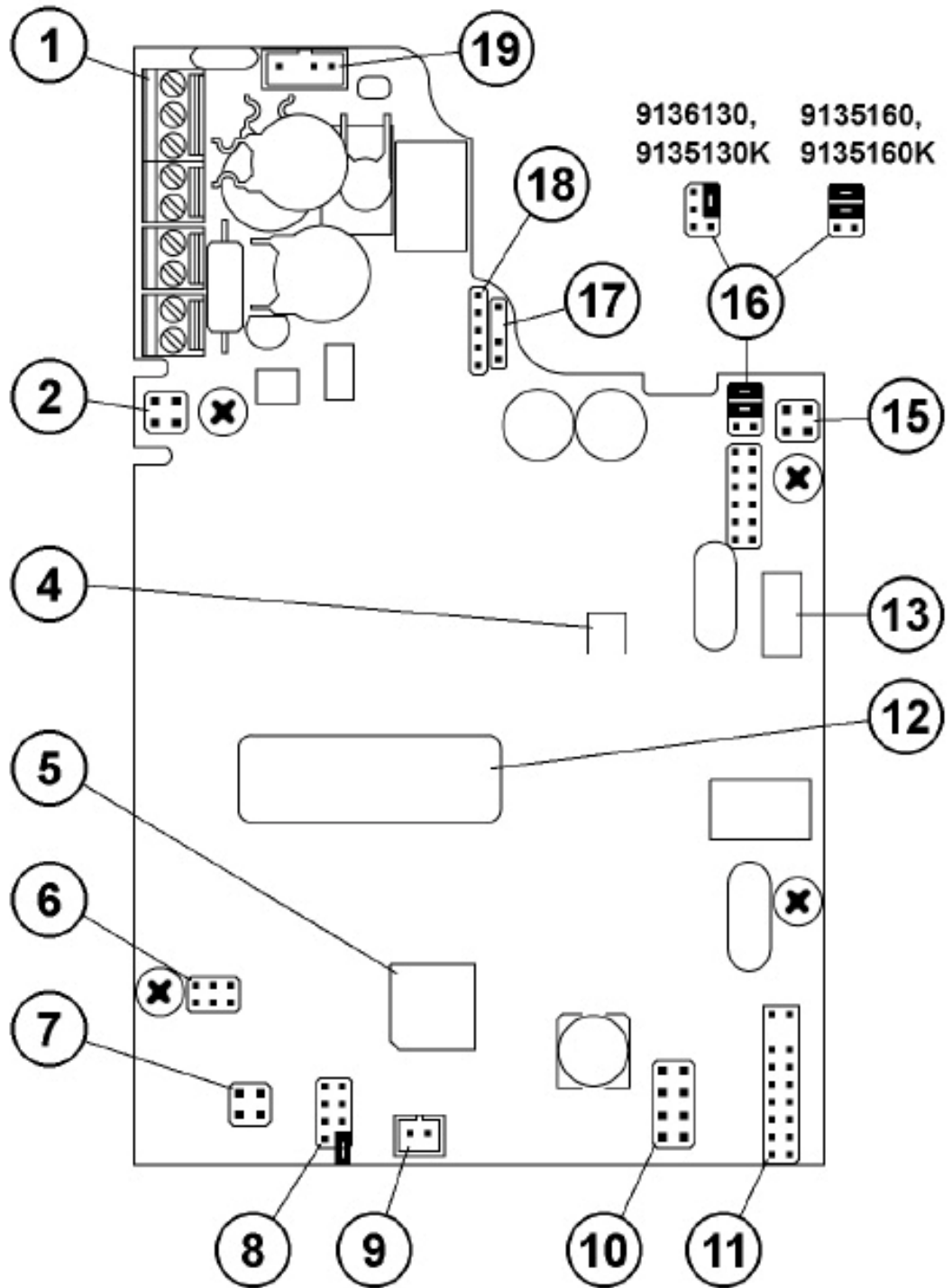
Fig.: PCB Layout, Version 14
