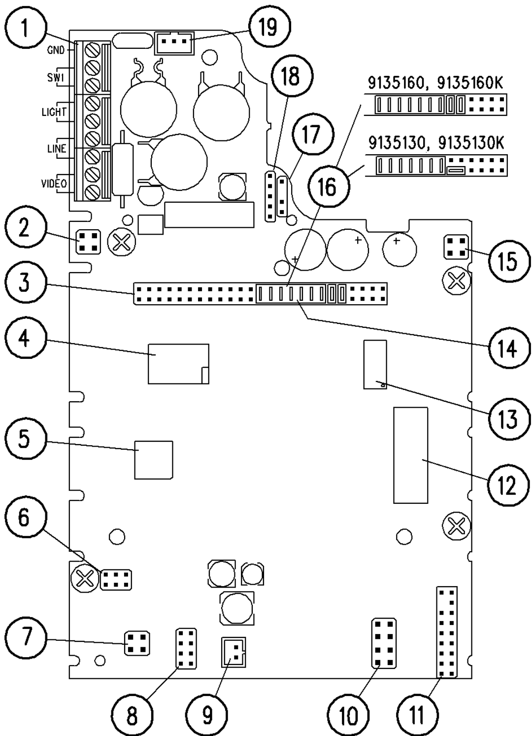
PCB Layout, Version 10
